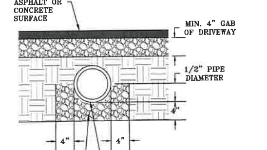
CROSS-SECTION A-A
