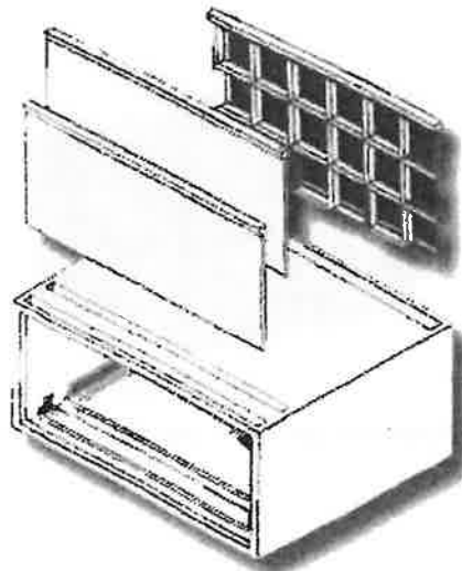
FIGURE 1—FLOOD FLAP ® AUTOMATIC FLOOD VENT
